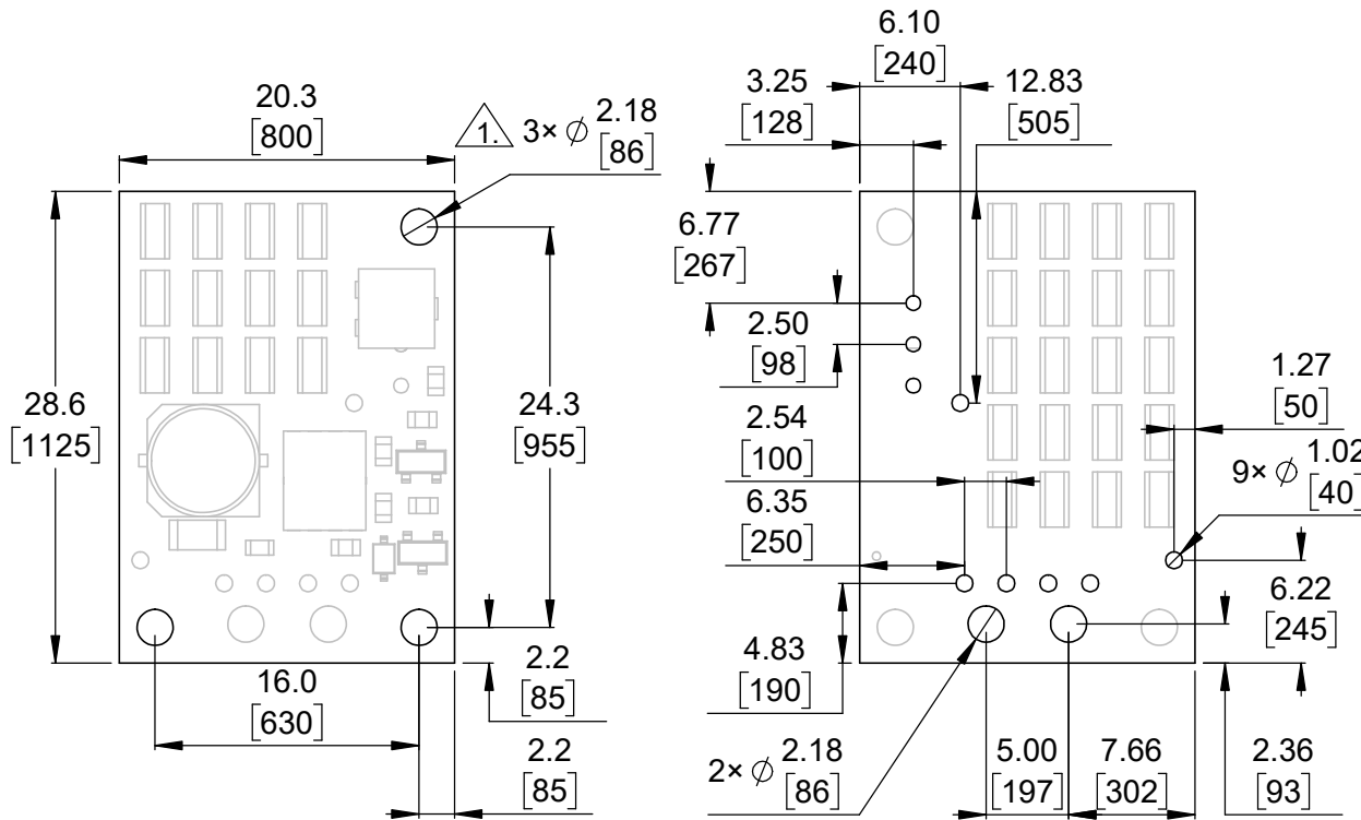
1 Board dimensions (top view) Scale 2:1
