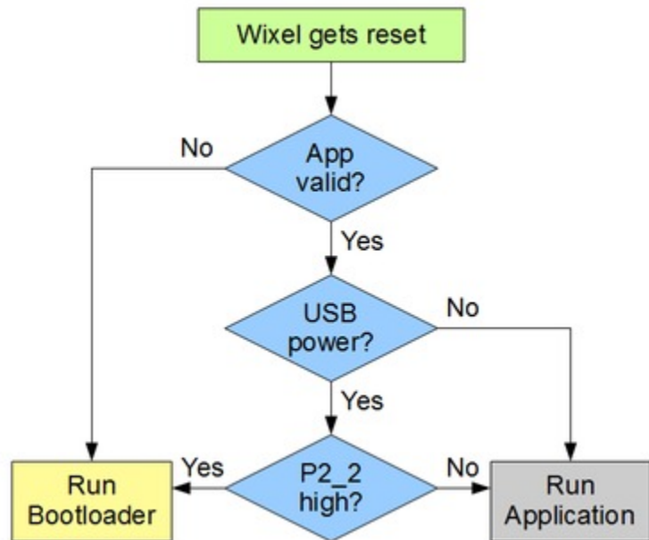
When the Wixel resets, it uses this procedure to decide whether to run the bootloader or the app.
