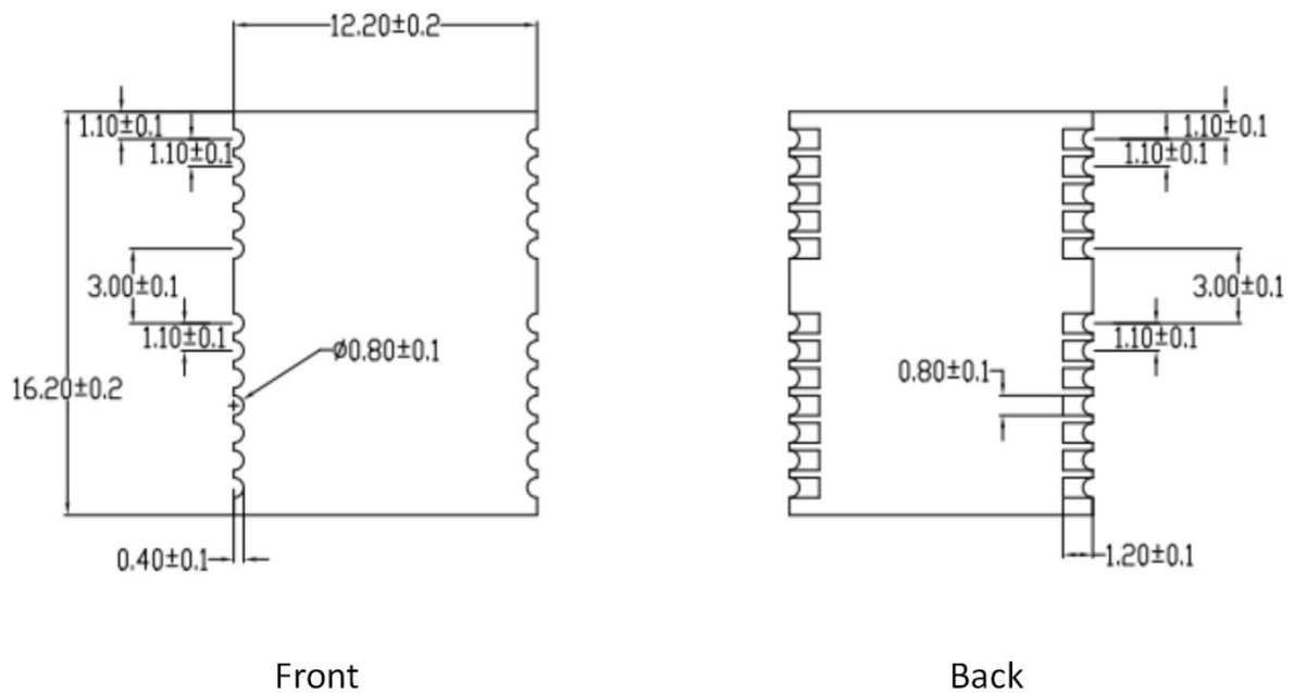
Figure 3 dimensions
