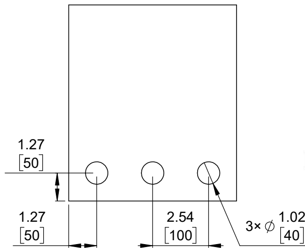
② Connector callouts (bottom view) Scale 6:1
