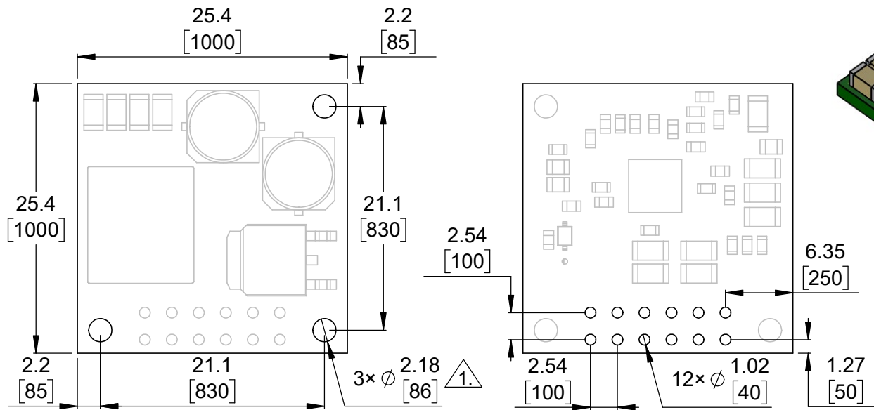
1 Board dimensions (top view) Scale 2:1
