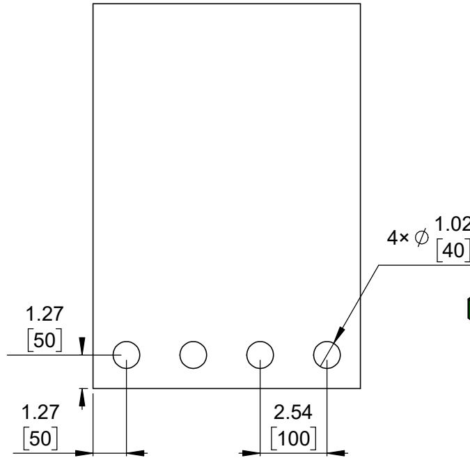
2 Connector callouts (bottom view) Scale 5:1
