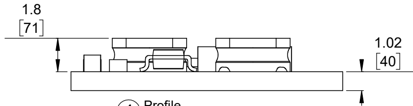
4 Profile Scale 5:1
