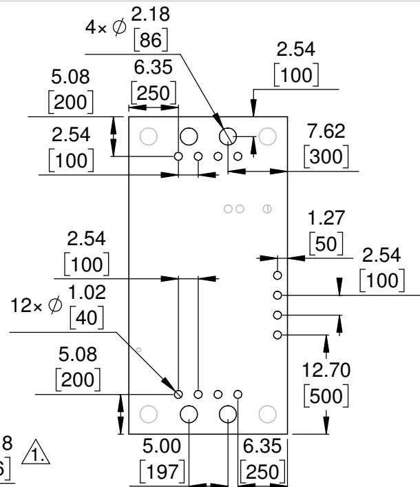
② Connector callouts (bottom view) Scale 3:2
