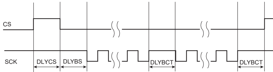
Figure 37-5. Programmable Delay
