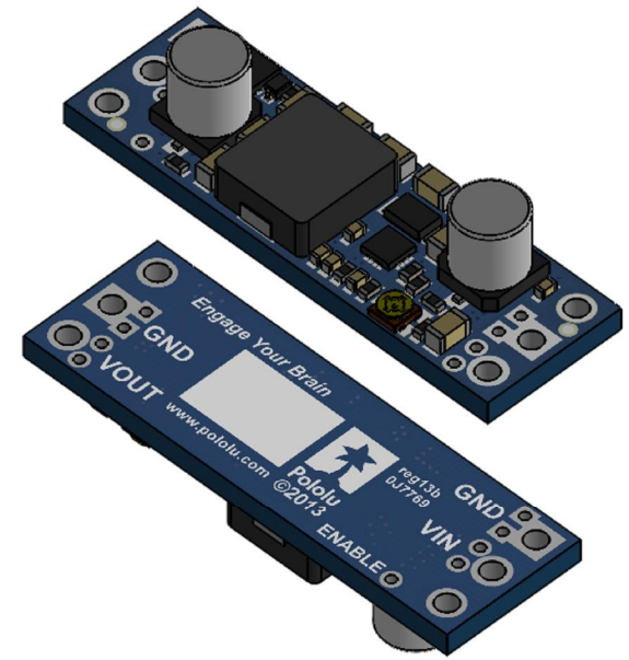
③ Isometric view Scale 3:2
