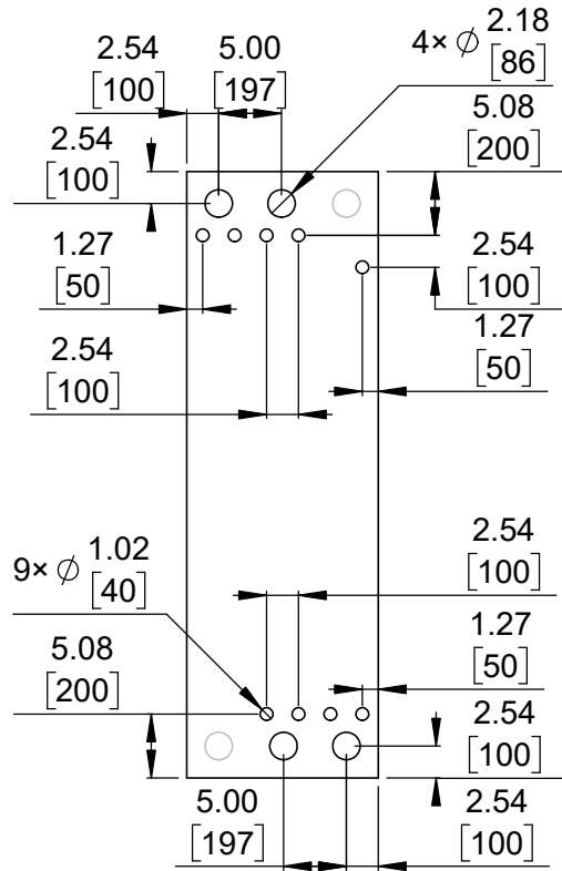
② Connector callouts (bottom view) Scale 3:2
