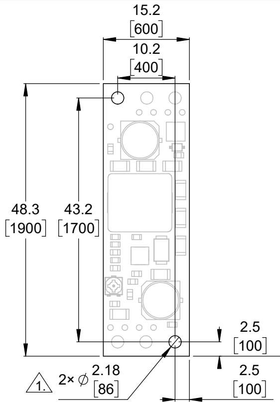
① Board dimensions (top view) Scale 3:2
