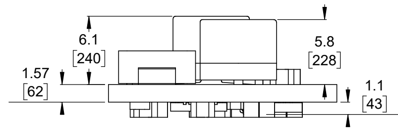
④ Profile Scale 3:1
