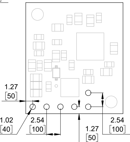
② Connector callouts (bottom view) Scale 3:1
