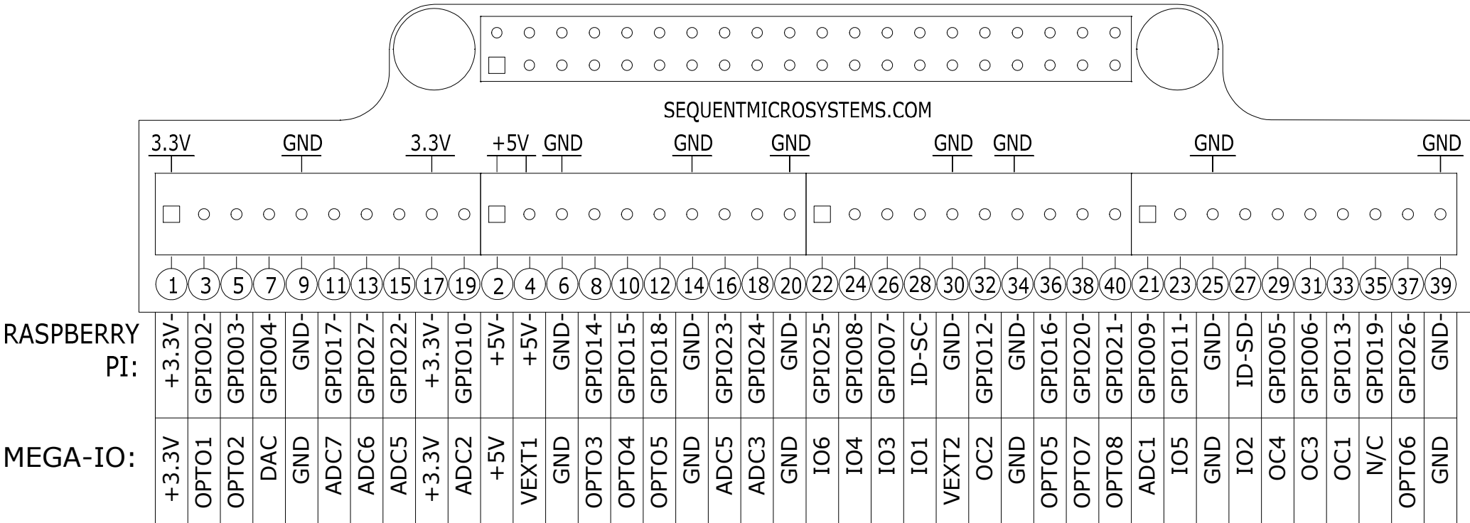
RASPBERRY PI/MEGA-IO BREAK-OUT CARD PINOUT
